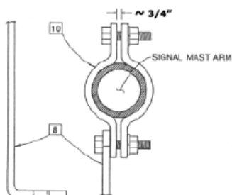
Optional Sign Mounting
